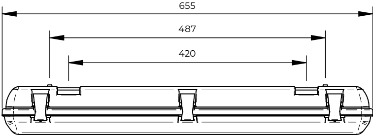
Dimensions (mm)
