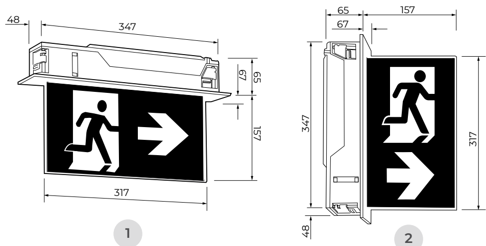
Dimensions (mm)
