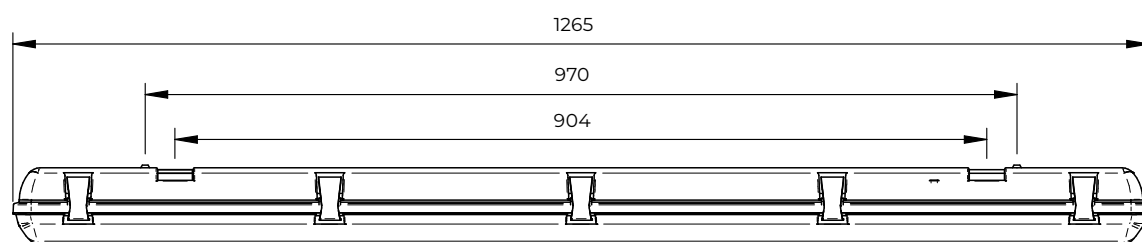
Dimensions (mm)
