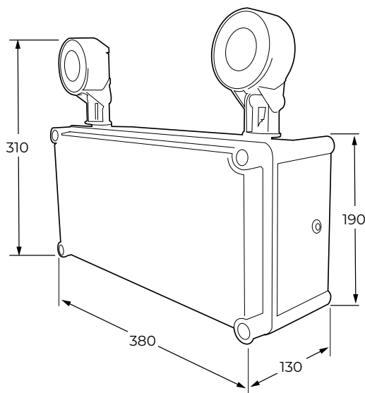
Dimensions (mm)
