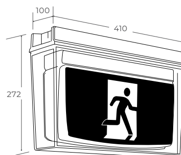
Dimensions (mm)
