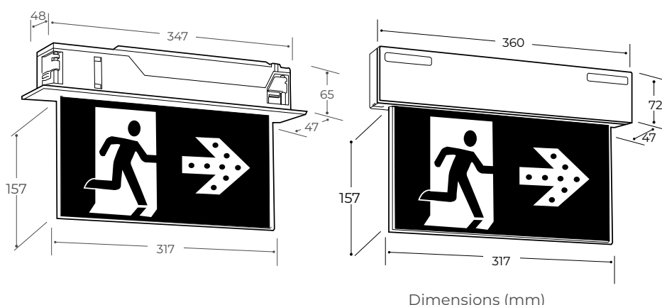
Dimensions (mm)
