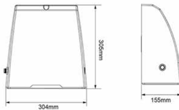
Dimensions (mm)
