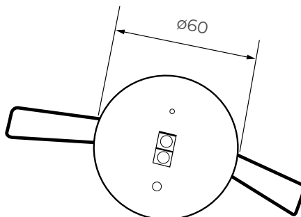
Dimensions (mm)
