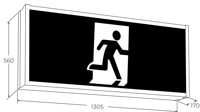
Dimensions (mm)
